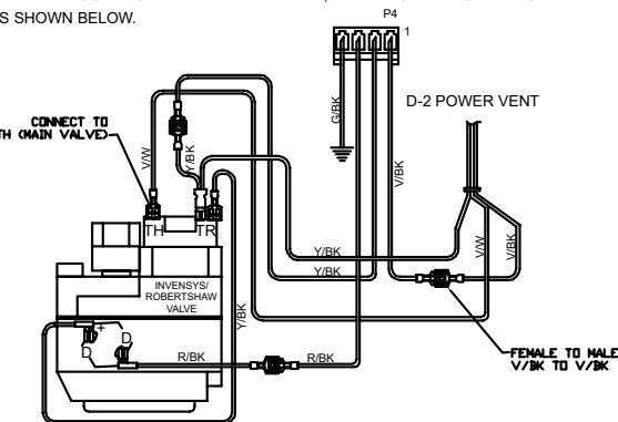
Figure 30. Connection Diagrams (206, 266, 268, 336, 406, 408) UNCONTROLLED DOCUMENT IF PRINTED
