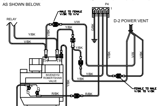
Figure 29. Connection Diagrams (207, 267, 337, 407) UNCONTROLLED DOCUMENT IF PRINTED
