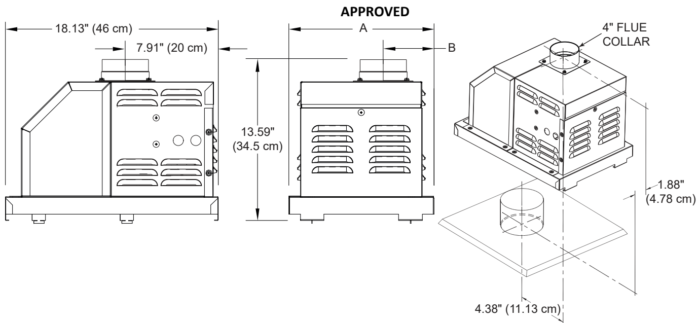
Figure 2. Dimensions
