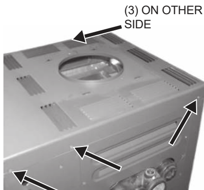
Figure 5. Screw Locations
