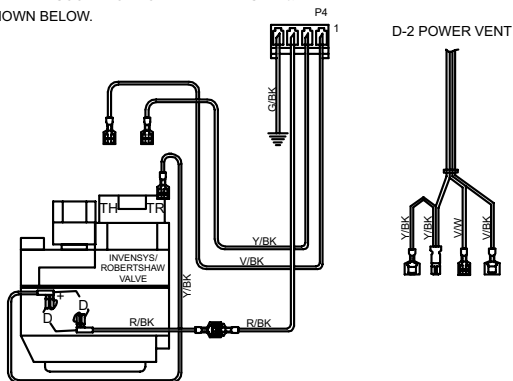
Figure 30. Connection Diagrams (206, 266, 268, 336, 406, 408) UNCONTROLLED DOCUMENT IF PRINTED
