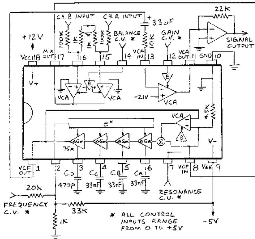
CEM3378 BLOCK & TYPICAL CONNECTION DIAGRAM
