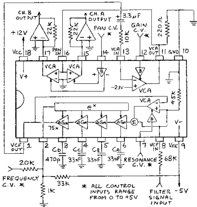
CEM3379 BLOCK & TYPICAL CONNECTION DIAGRAM
