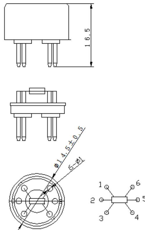
Fig1.Sensor Structure
