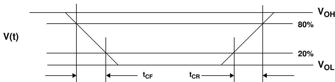
Figure 6. Voltage Waveforms
