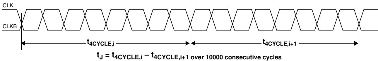
Figure 11. Short-Term Jitter
