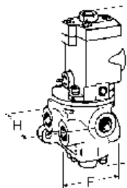
4/2 Valves
