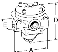
3/2 Valves
