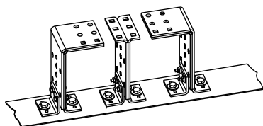
RTL Terminal Pad Kit
