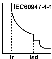
MicroLogic 2.2M and 2.3M Trip Units Ii=4800A
