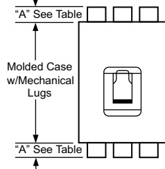
Crimp lugs or PDC connectors extension "A" past end of circuit breaker
