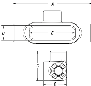
T Sand Cast Aluminum Form 7
