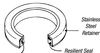
Resilient Sealing Material Locked in Steel Retainer
