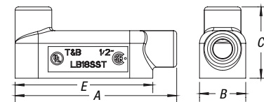
LB Form 8 Conduit Bodies with Covers
