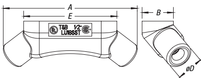
LU® Form 8 Conduit Bodies with Covers
