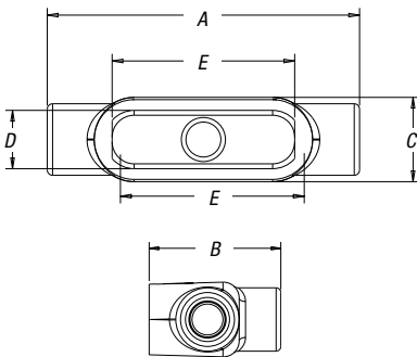
TB Sand Cast Aluminum Form 7
