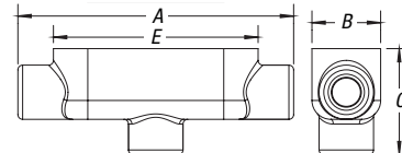
TB Form 8 Conduit Bodies with Covers
