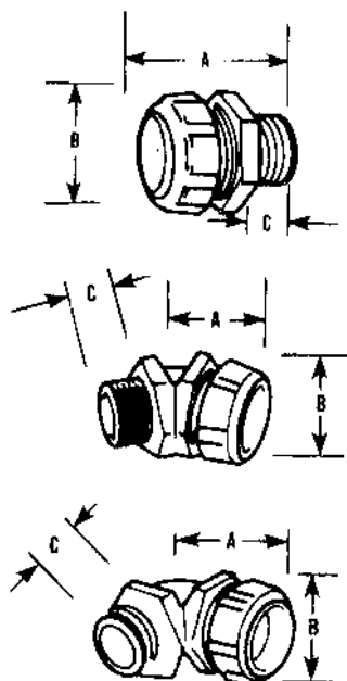
Fittings for Liquidtight flexible metal conduit with metric threads of PG Form (DIN 40430).
