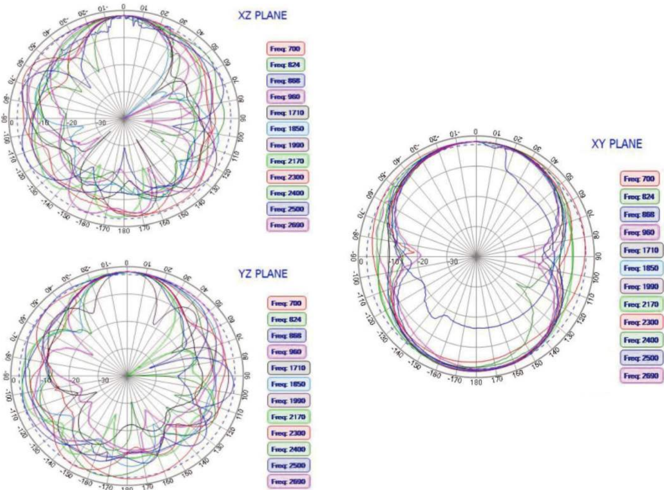
Radiation Pattern
