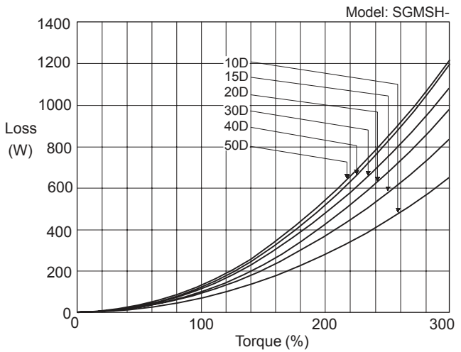
SGMSH Servomotors
