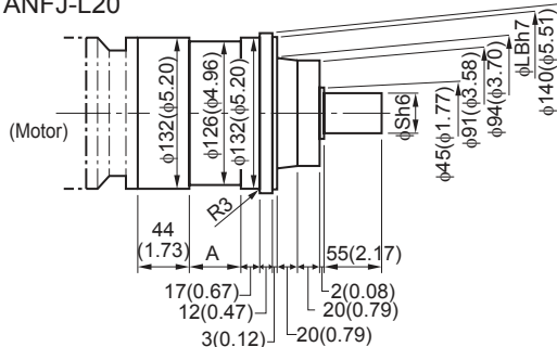
ANFJ-L20
