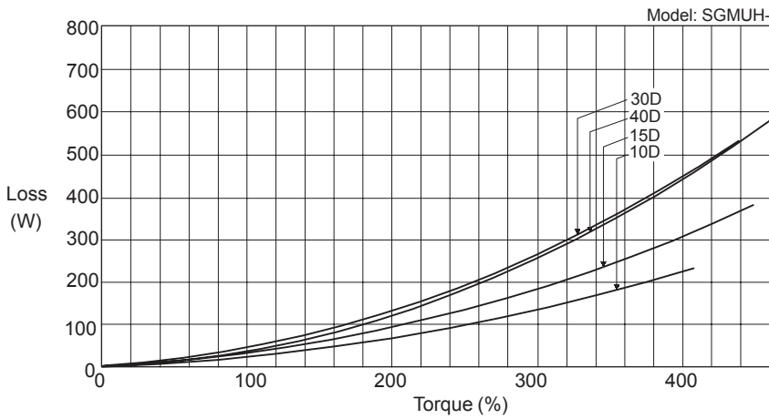
SGMUH Servomotors
