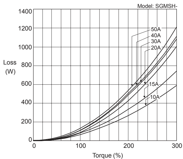
SGMSH Servomotors
