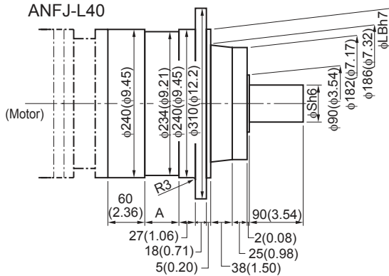
ANFJ-L40
