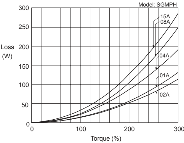
SGMPH Servomotors
