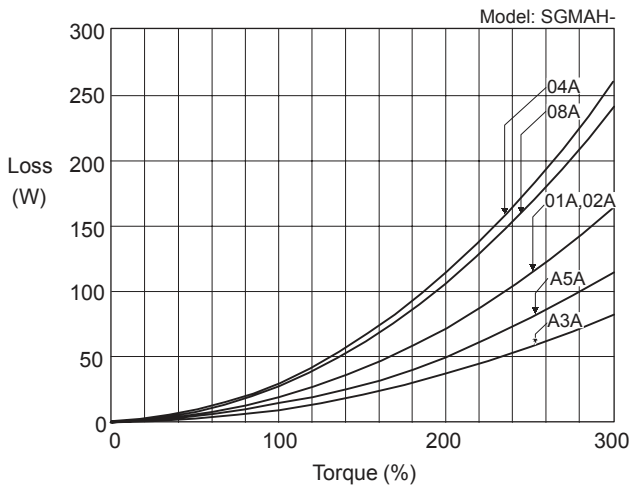
SGMAH Servomotors
