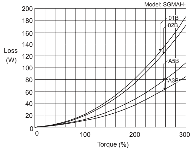
SGMAH Servomotors
