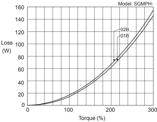
SGMPH Servomotors
