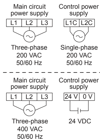
External Terminal Connector
