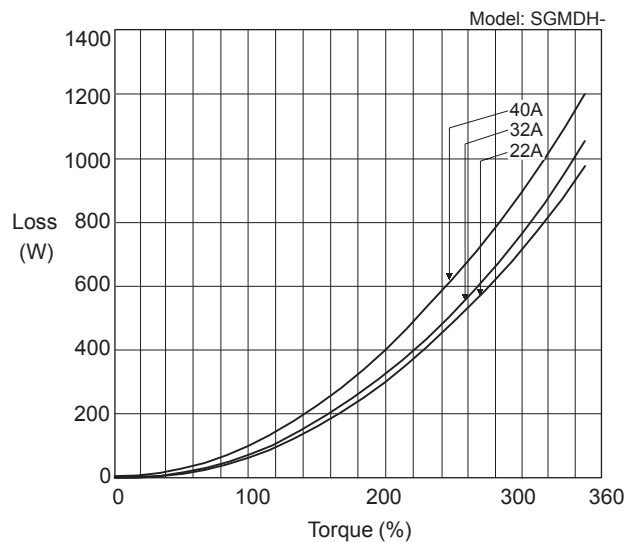
SGMDH Servomotors
