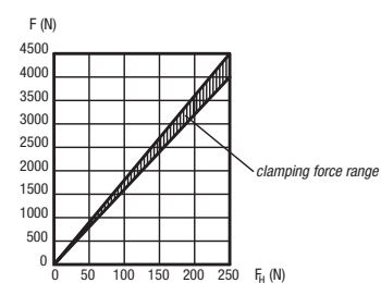
Force diagram
