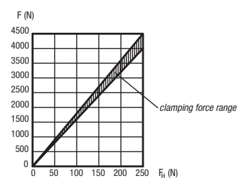
Force diagram
