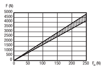
Force diagram
