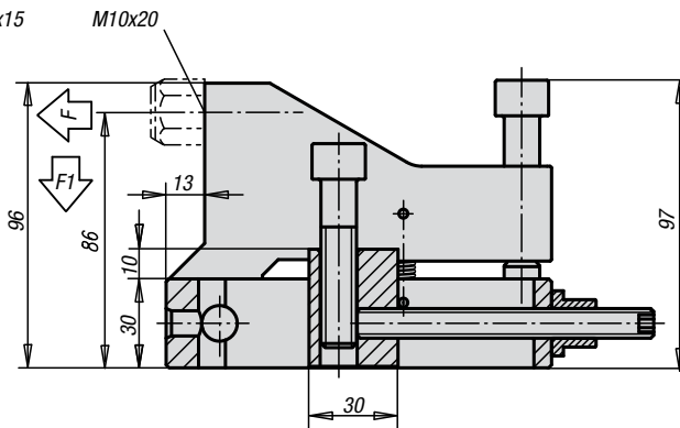
K0830.112 Side clamp
