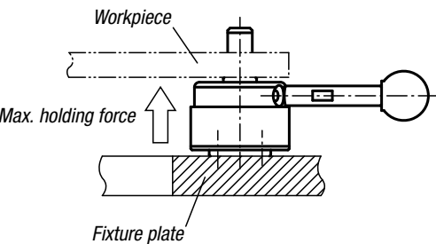
Holding forces for workpiece processing
