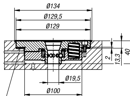
Installation without overhang
