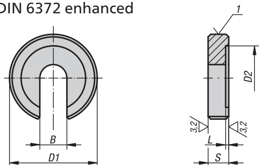
KIPP C-washers for fixtures DIN 6372 enhanced
