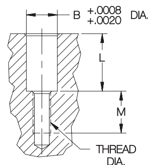
Installation Hole
