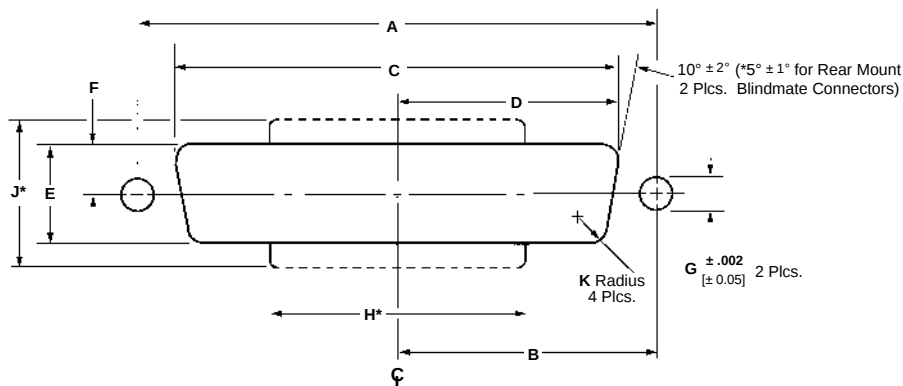
Panel Cutout
