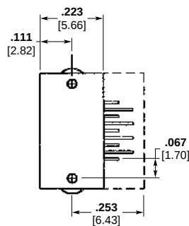
Horizontal Surface Mount
