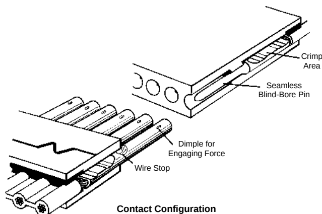
Contact Configuration
