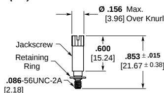
Part Number 5-1532137-8 Jackscrew Assembly High Profile (K) 096-0002-0010 M83513/5-06 (KM) S96-0002-0084
