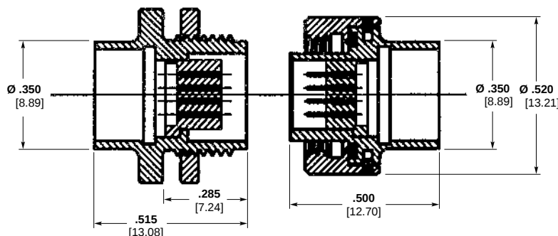
NCG044 — 44 Position Circular
