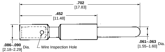
Part Number 083-0158-00R4 16 AWG Pin
