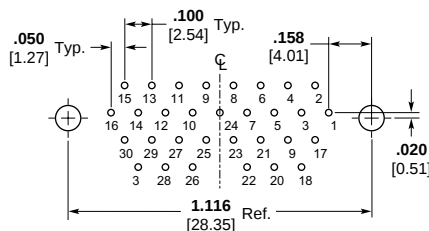
31 Contacts
