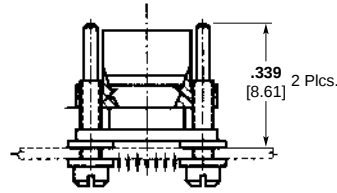
Metal Shell, 2 Row, DUALOBE, 15 Position Plug
