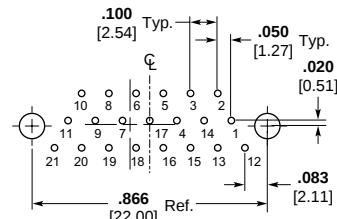
21 Contacts
