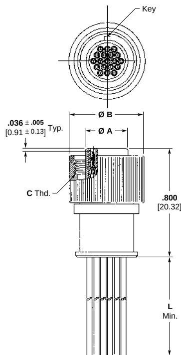
MTC Series Plug (19 Position Shown)
