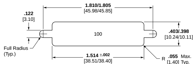
Rear Mounting
