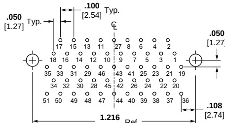
51 Contacts
