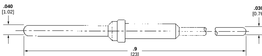
Pin Part Number 194081-1
