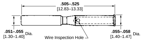
Part Number 082-0461-00Y9 22 AWG Socket
