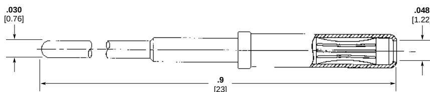
Socket Part Number 194083-1
