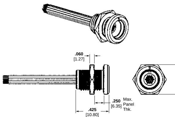
19 Position Flush Mount Receptacle (Shown)
