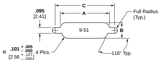
Figure 2 Rear Mounting
