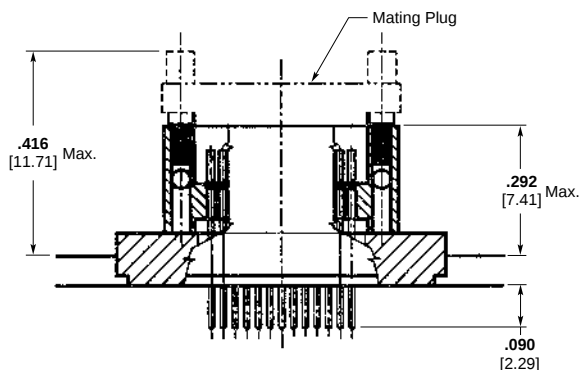
Two Row, Glass Seal, Receptacle
