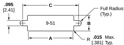
Figure 1 Front Mounting
