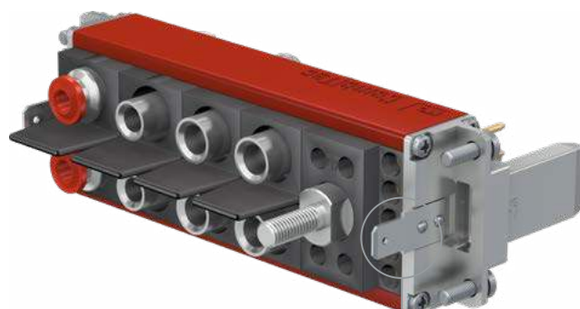
End pieces with contact spring and flat plug connection
