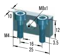
Mounting Block
