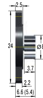
Dims. in ( ) without gear
