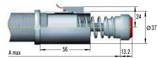
Switch Stop Collar
