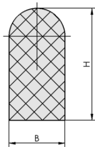
Design data DR 141/149x6 MOS NK-20
