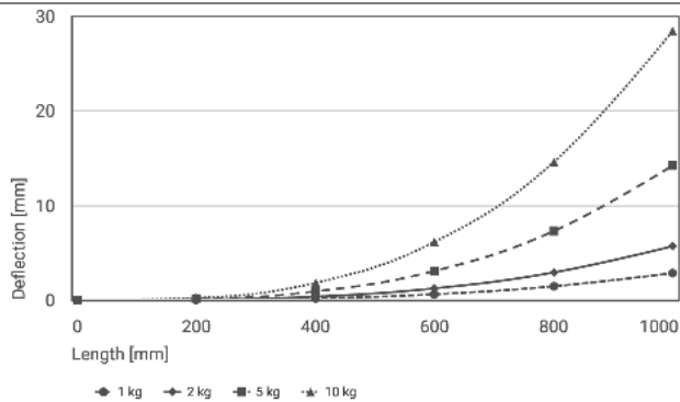
Deflection pipes 25 x 5 mm
