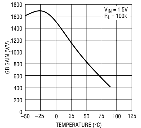
“Gain Block” Gain
