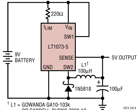
9V to 5V Step-Down Converter
