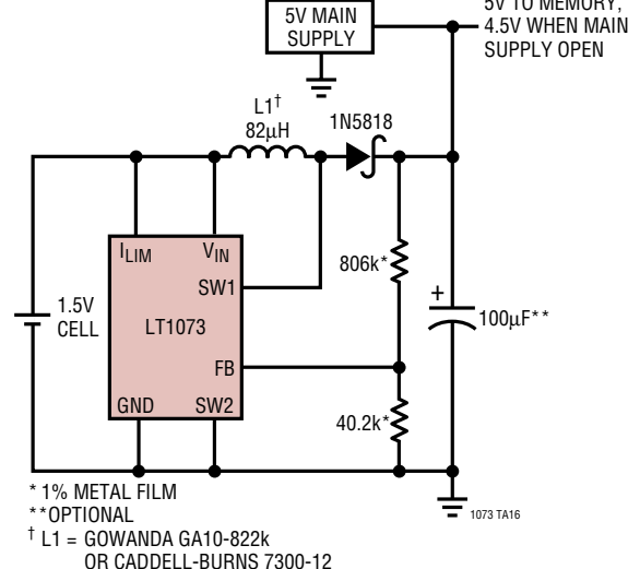
Memory Backup Supply
