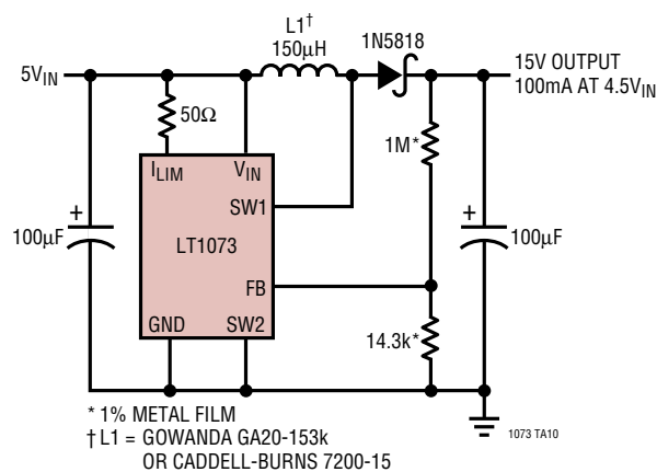
5V to 15V Step-Up Converter
