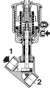
NC function, entry above the disc, 63 mm actuator
