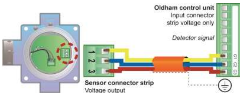
Figure 11: connections for a 3-wire OLC 100 type detector
