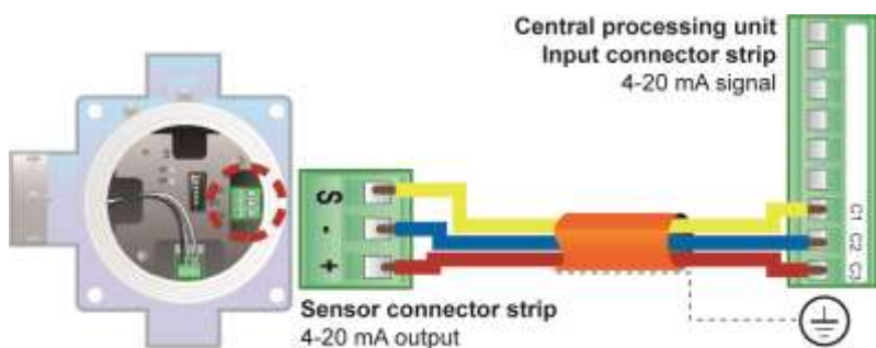
Figure 10: connections for a 3-wire 4-20 Ma detector
