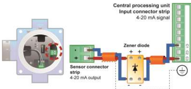
Figure 9: connections for an intrinsically safe, 2-wire 4-20 Ma detector with a Zener diode
