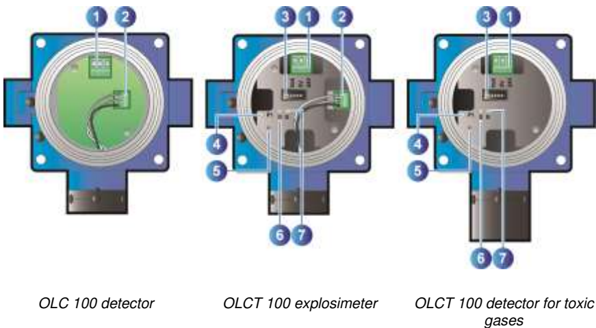
Figure 2 : internal view of the detectors
