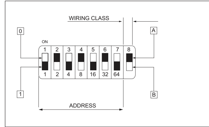
Fig 3. DIL Switch
